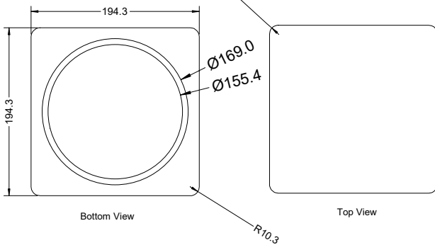
Hopper cover
